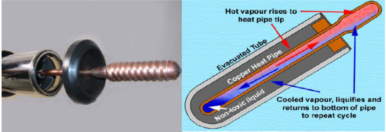
Structure of heat pipe with glass tube:
